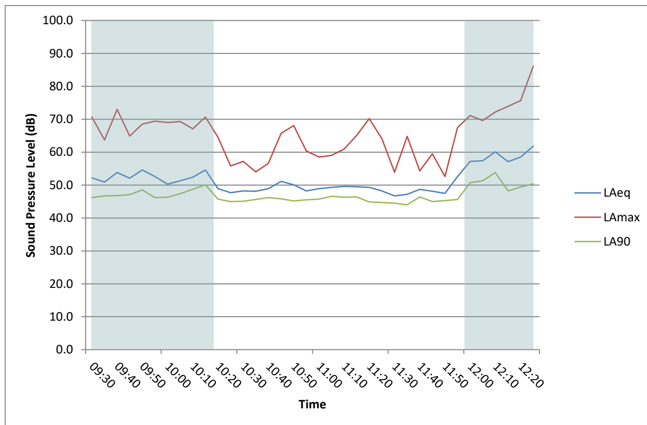
Figure 6.1: Sound pressure level at fixed location, F1
