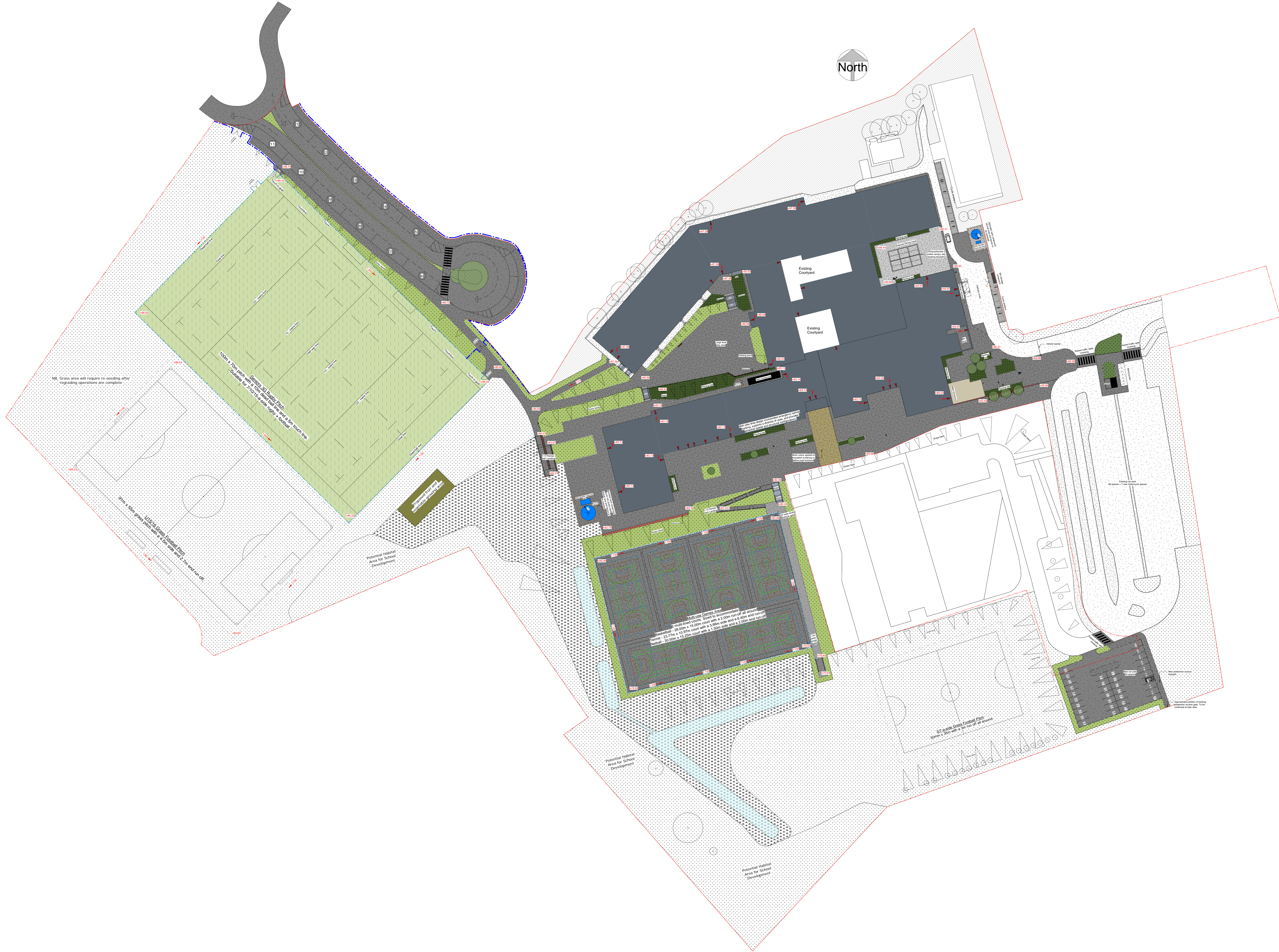
0900 - External Works General Arrangement - Whole Site 1:500
