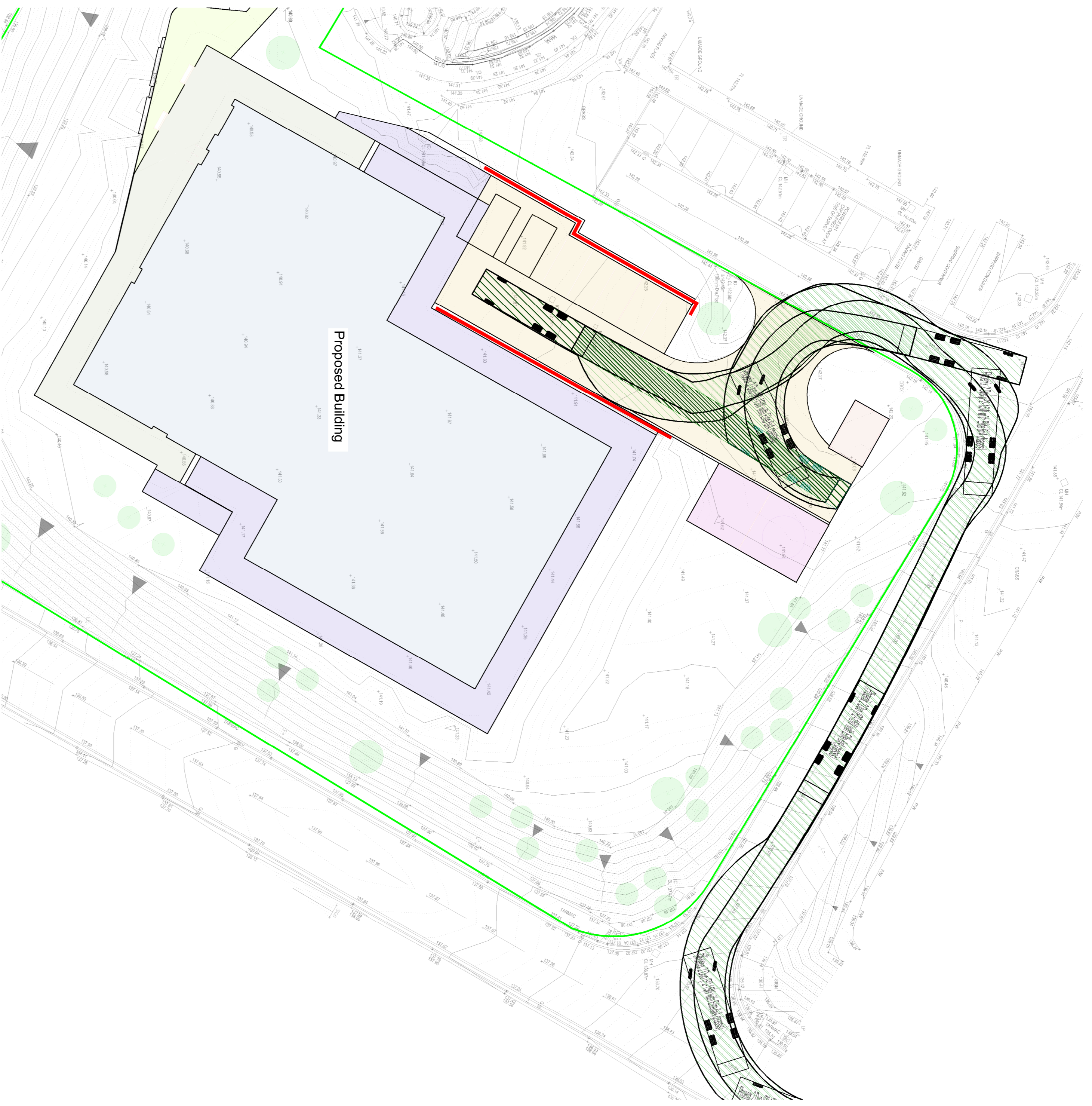
Vehicle Tracking Refuse Vehicle (Scale 1:250)
